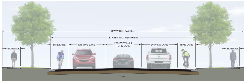
Alternative C: Two Way Left Turn Lane with Bike Lanes
