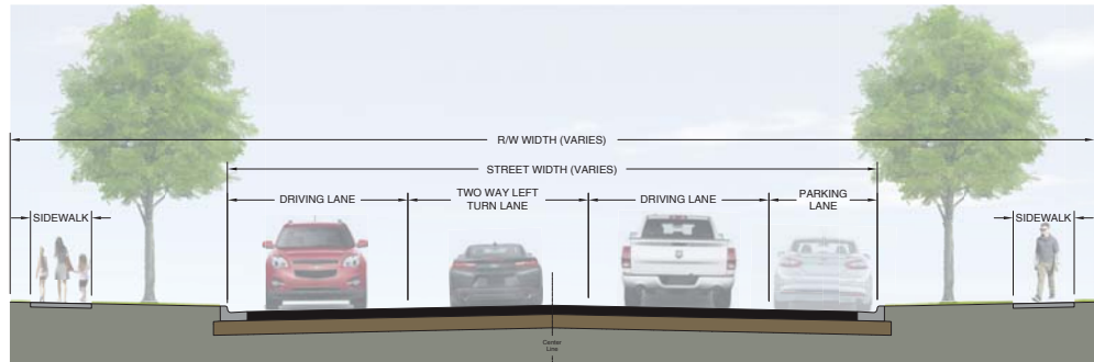
Alternative D1: Two Way Left Turn Lane with Parking Lane Right
