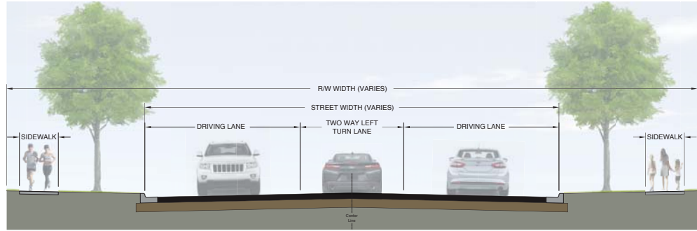
Alternative B: Two Way Left Turn Lane
