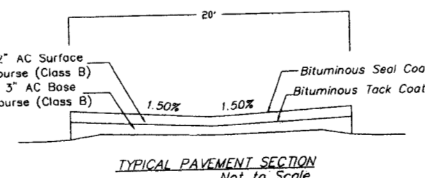
TYPICAL PAVEMENT SECTION NOT TO SCALE
