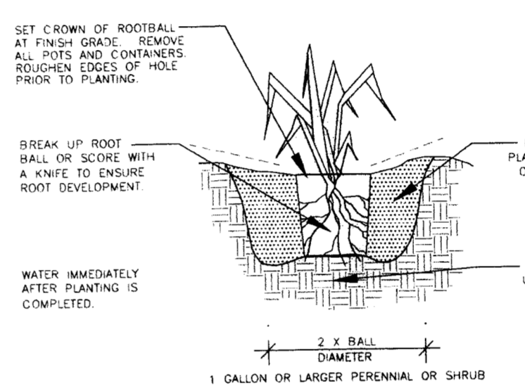
SHRUB/PERENNIAL PLANTING DETAIL TYPICAL FOR ALL SHRUBS AND PERENNIALS
