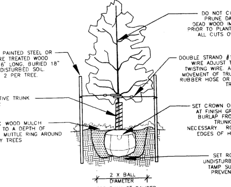
TREE PLANTING DETAIL TYPICAL FOR ALL DECIDUOUS, SINGLE-TRUNK, TREES
