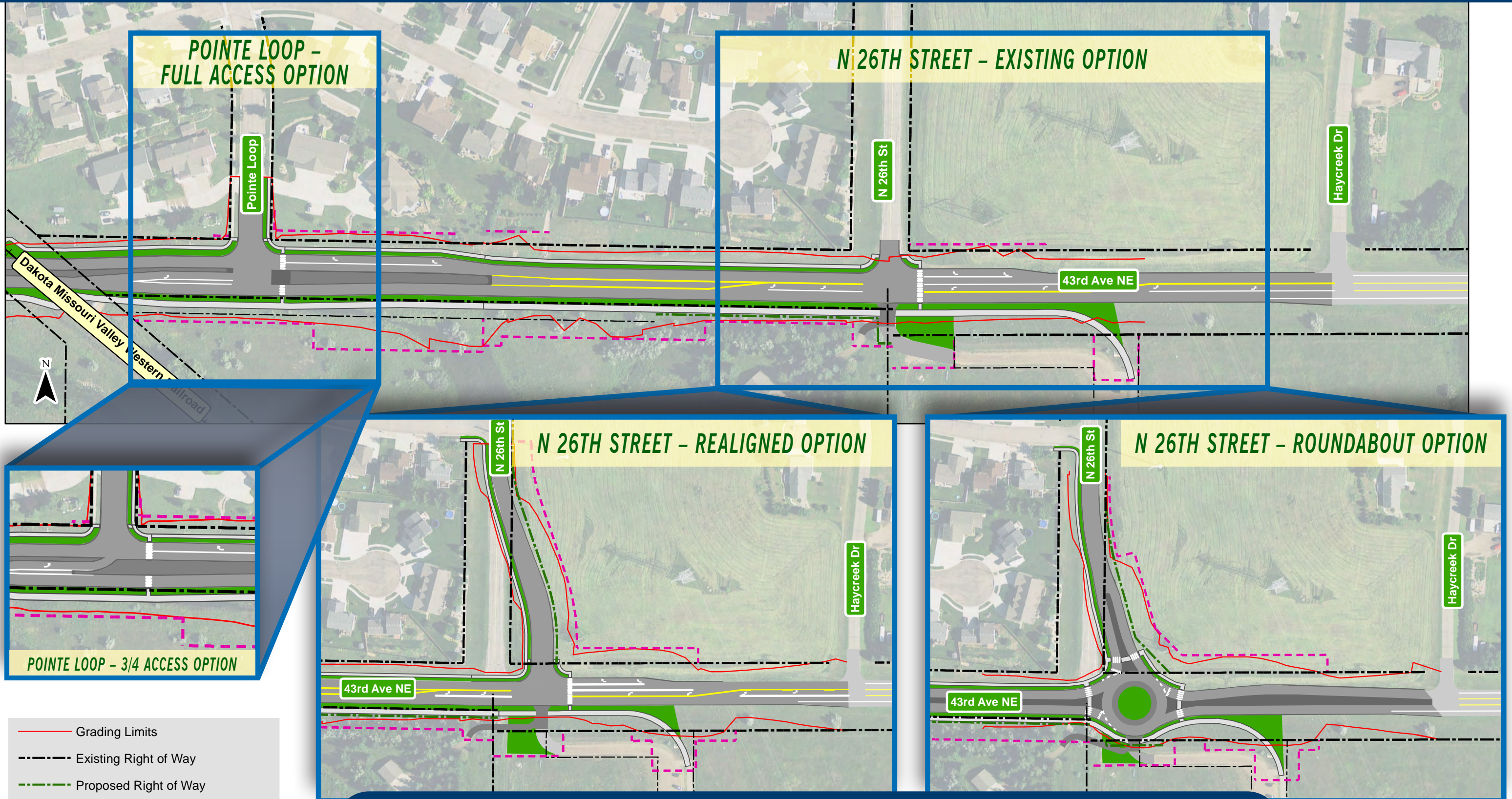
EXHIBIT 5. POINTE LOOP & N 26TH STREET OPTIONS
